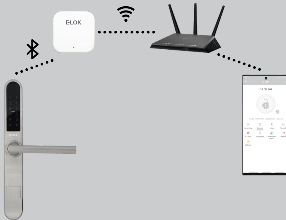
Bluetooth + E-LOK Gateway Remote access add-on
